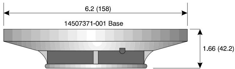
Fig. 3: Low Profile Sensors and Mounting Base
